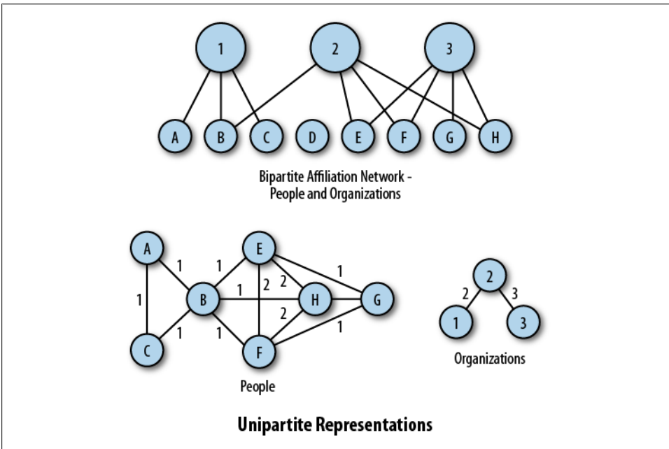
Figure 5-4. Creating an affiliation network from a 2-mode network
