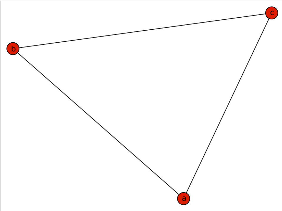
Figure 3-1. Simple graph
