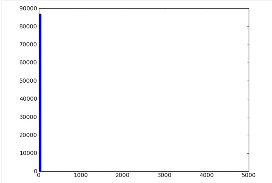
Figure 3-3. Degree histogram
