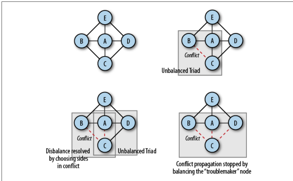
Figure 4-14. Conflict propagation
