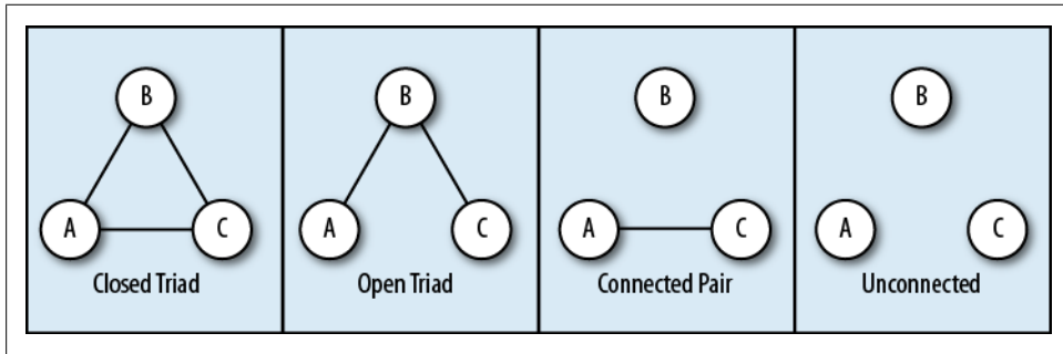
Figure 4-2. Triad shapes
