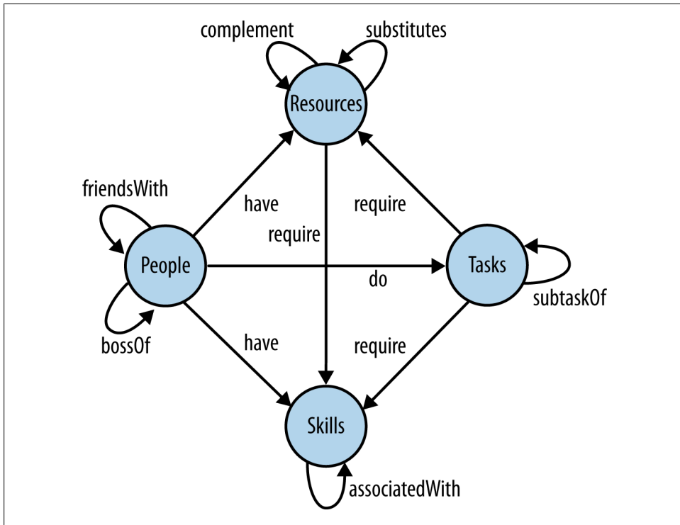
Figure 5-8. Entity-relationship diagram of a simple organization
