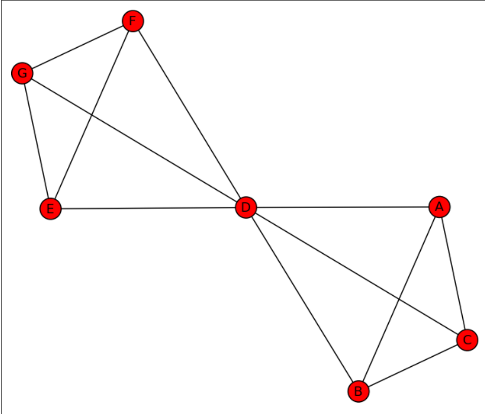
Figure 3-7. Bow-tie network
