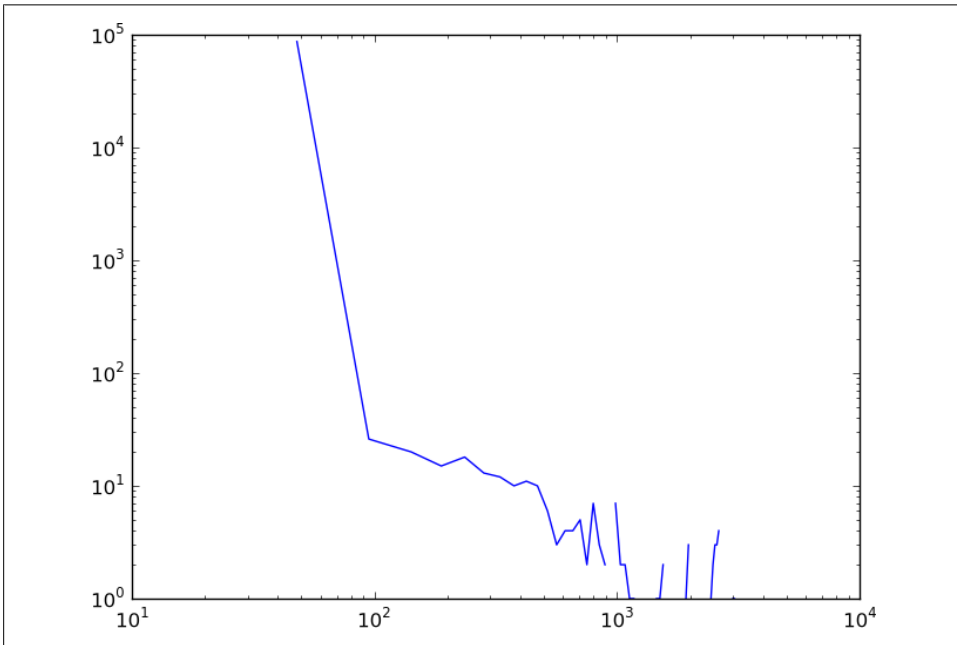
Figure 3-4. Degree histogram (LogLog Plot)
