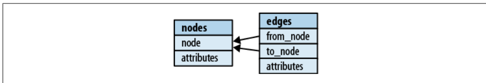
Figure 7-2. Database schema for storing network data
