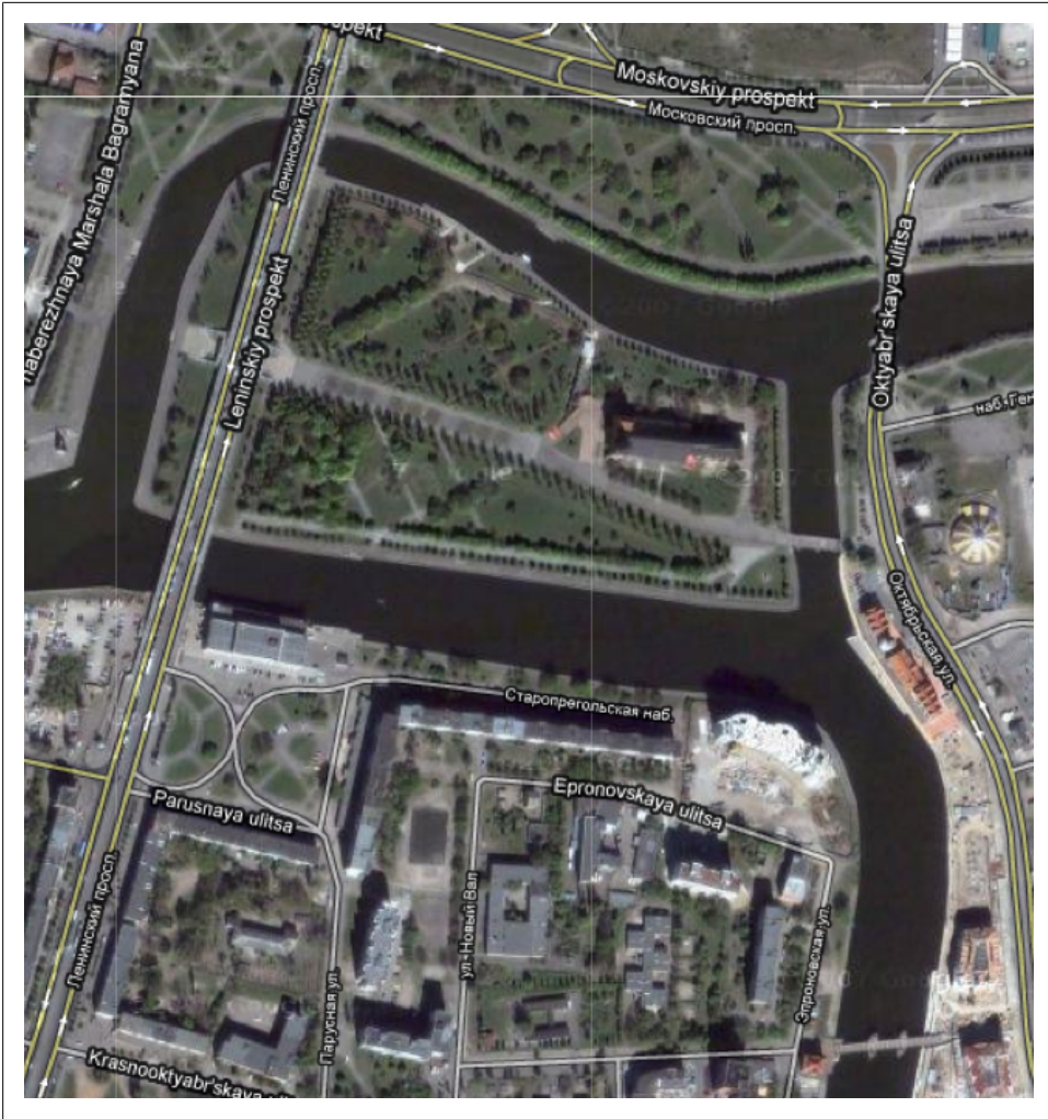
Figure 2-2. The Five Bridges of Kaliningrad—a modern view. This is all that remains after World War II, but Euler's theorem still holds
