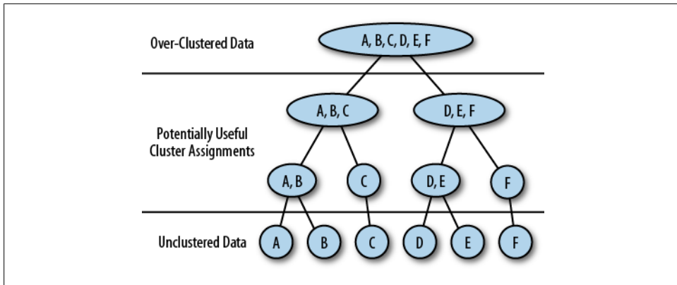
Figure 4-10. Hierarchical clustering
