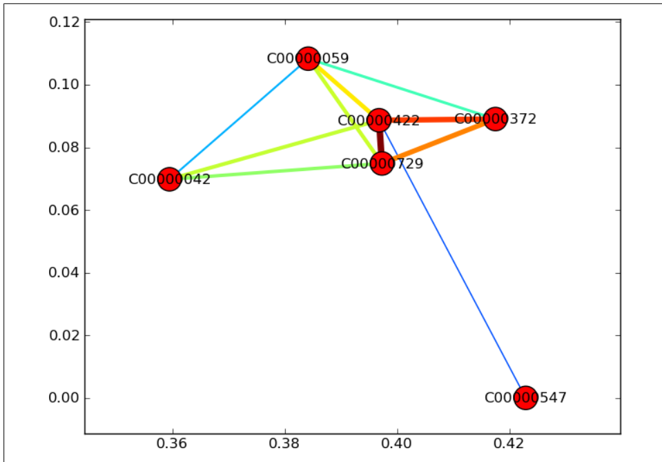
Figure 5-5. Sample affiliation network of PACs
