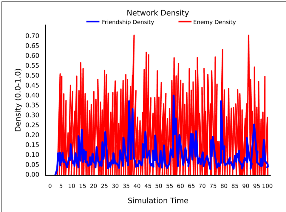
Figure 4-15. Conflict cascades occur—Rule 2 activated
