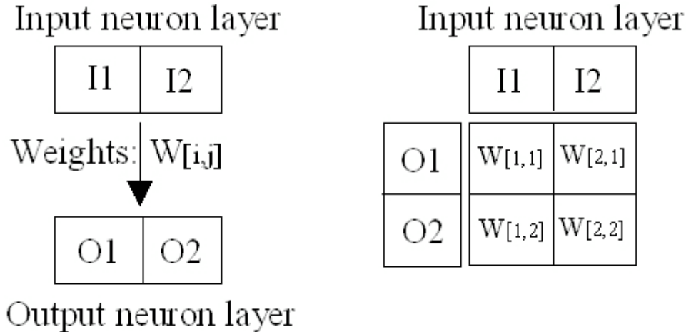
Figure 5.3 Two views of a two layer neural network; the view on the right also shows the connection weights between the input and output layers.
