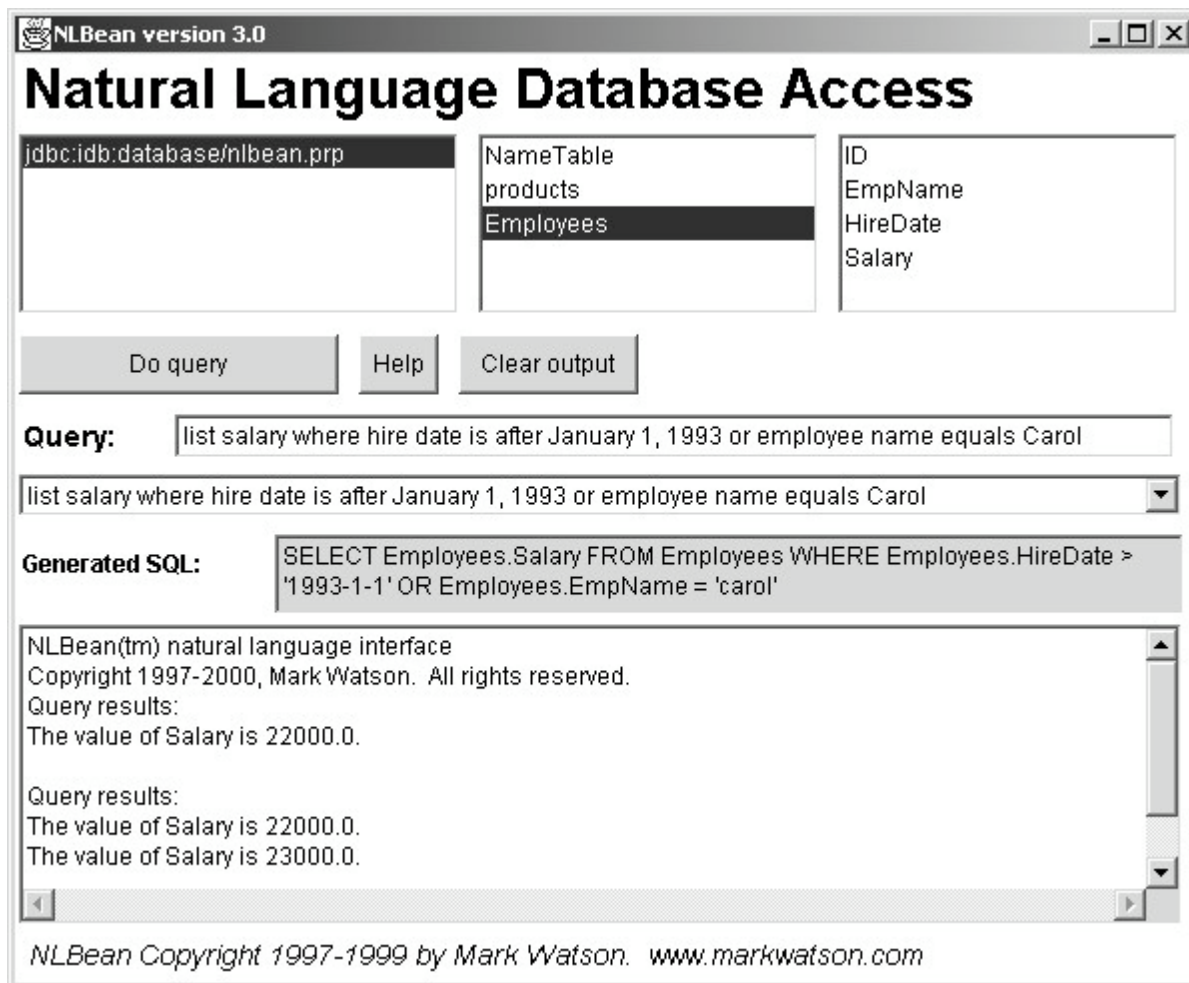
Figure 2.3 the NLBean
