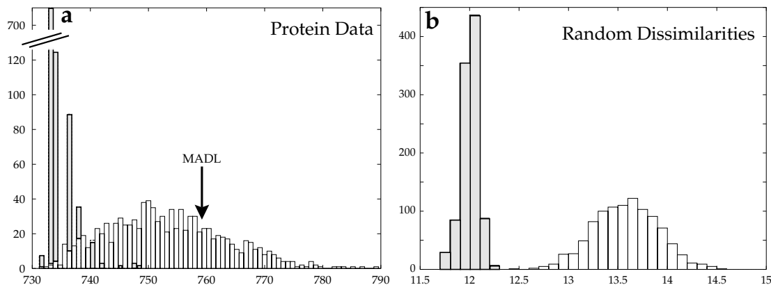
Figure 1: Histograms of clustering costs for a protein data set (a) and a random clustering instance (b) . The gray and white bins denote the results of optimization with deterministic annealing and gradient descent, respectively. The Mean Average Dissimilarity Linkage solution has costs of \mathcal{H}^{\text{pc}} = 759.1 .
