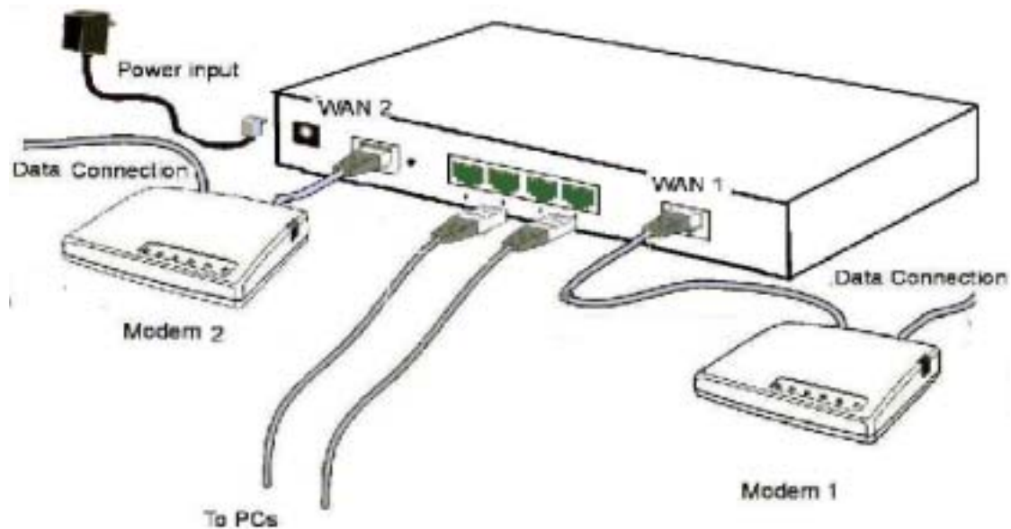
Figure 2-4: Installation Diagram LB-2
