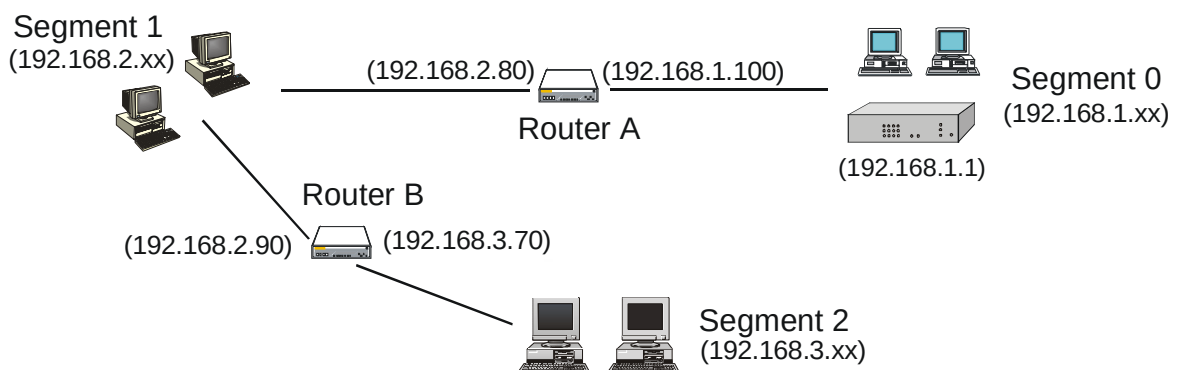
Figure 8-2: Routing Example
