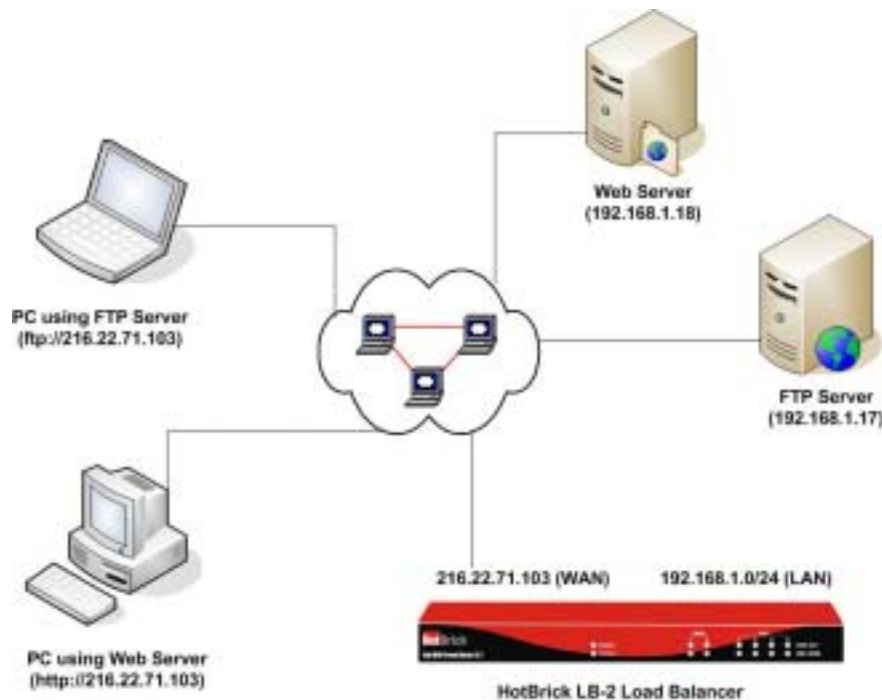
Figure 4-2: Virtual Servers
