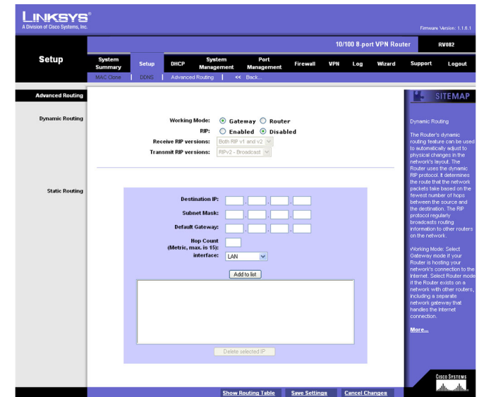
Figure 5-21: Setup Tab - Advanced Routing
