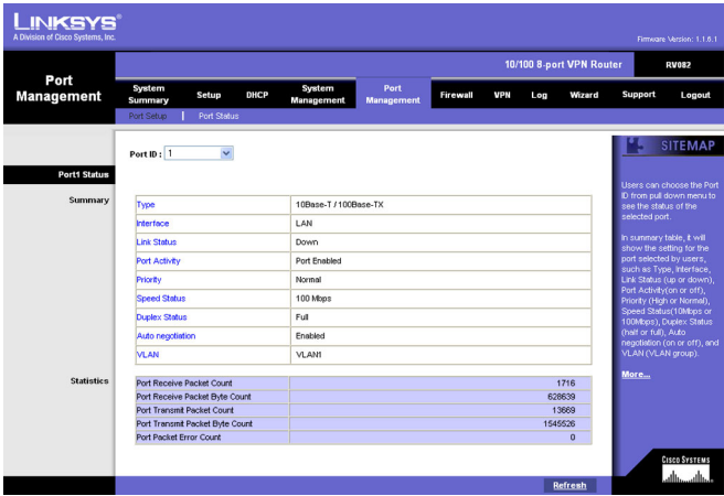
Figure 5-36: Port Management Tab - Port Status
