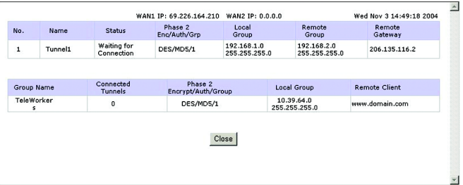
Figure 5-43: VPN Tab - Summary Detail
