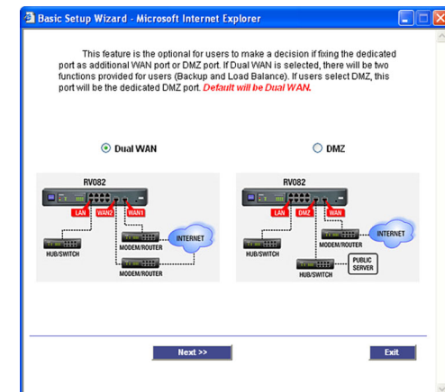
Figure 5-61: Basic Setup Wizard - Dual WAN or DMZ
