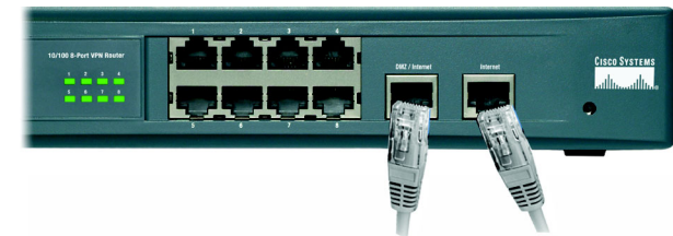
Figure 4-3: Connect the Internet and DMZ/Internet
