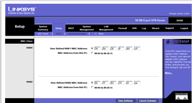
Figure C-4: MAC Address Clone
