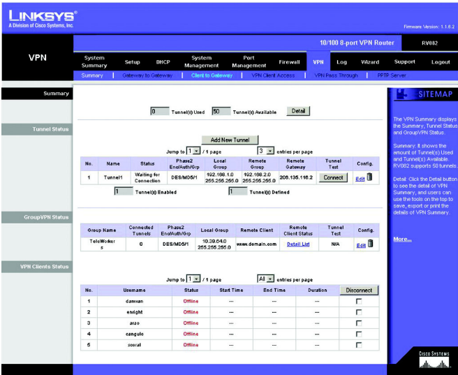
Figure 5-42: VPN Tab - Summary
