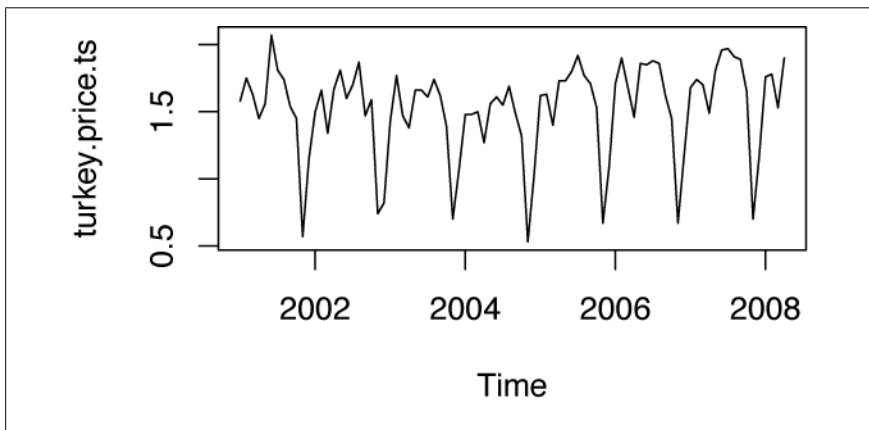
Figure 14-5. Time series plot
