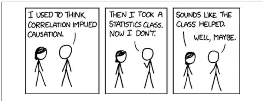
Figure 16-1. Correlation
