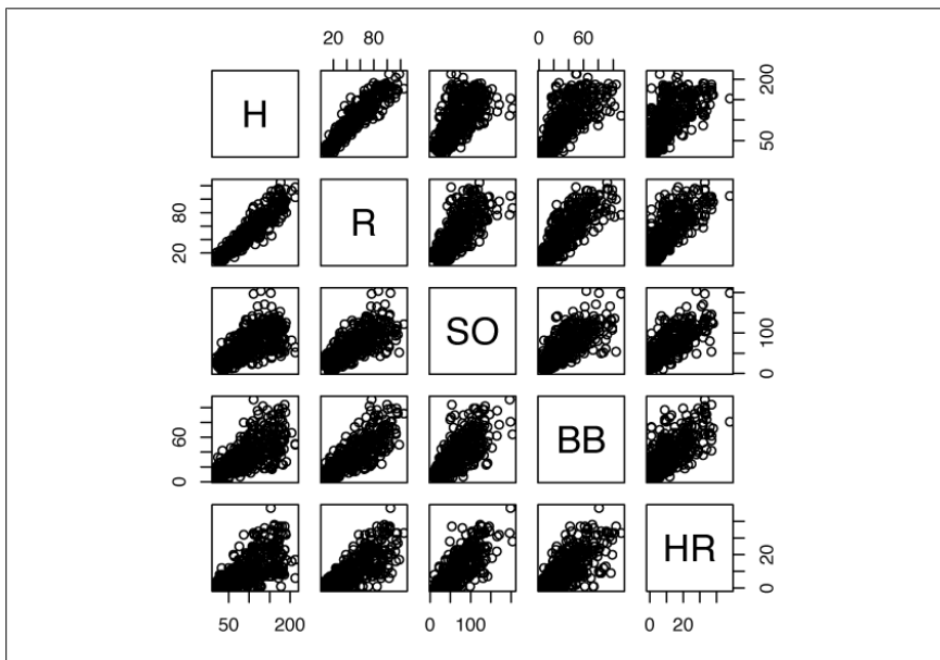
Figure 14-4. Pairs example
