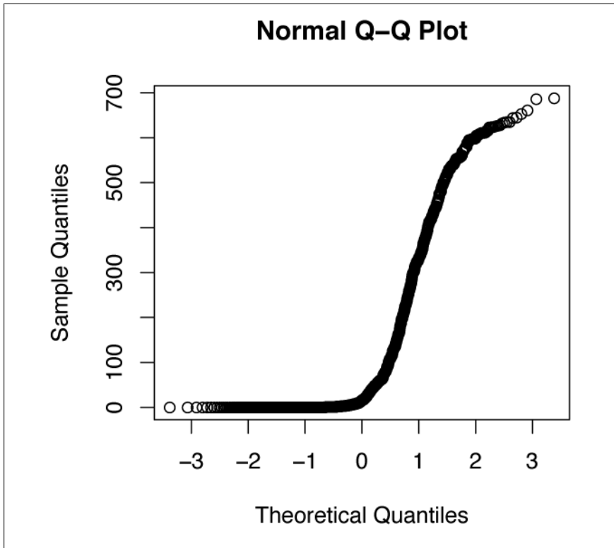
Figure 14-21. Quantile-quantile plot
