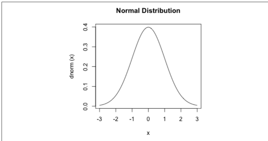
Figure 17-1. Normal distribution
