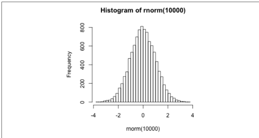
Figure 17-3. Histogram of 10,000 random values from a uniform distribution
