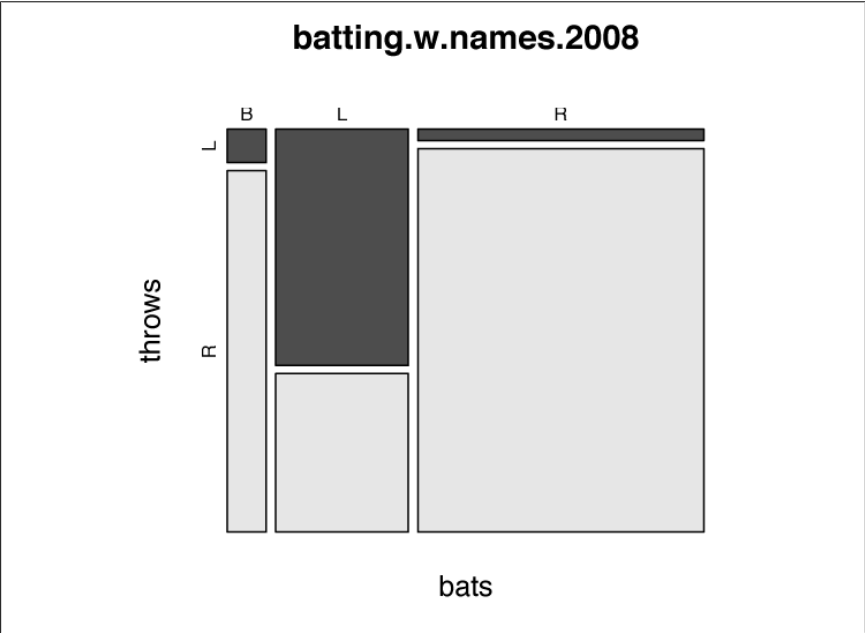
Figure 14-12. Mosaic plot
