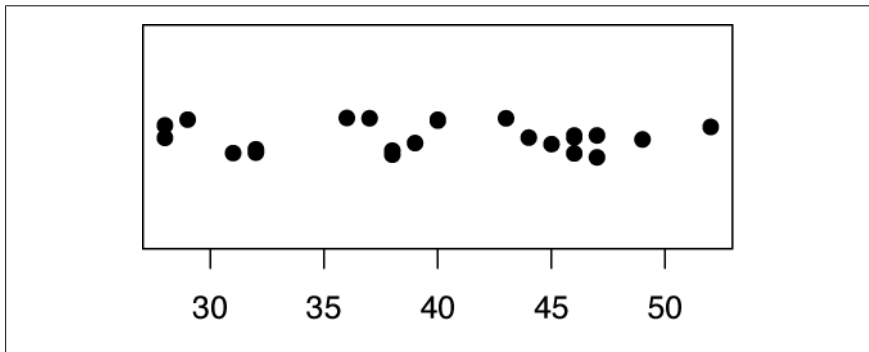
Figure 3-3. Strip chart showing field goal attempt distances
