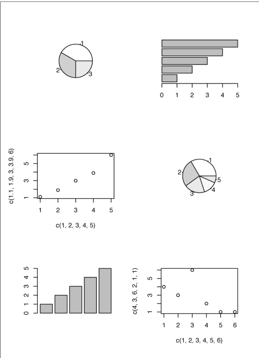
Figure 14-25. Multiple-figure example
