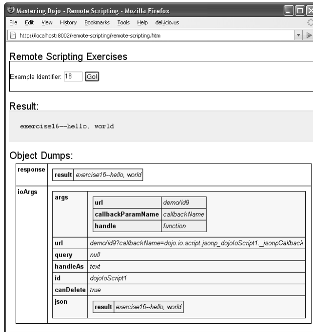
Figure 8.7: dojo.io.script.get with a callback
