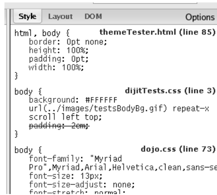
Figure 16.4: Firebug CSS window
