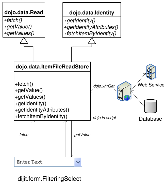
Figure 10.1: dojo.data architecture
