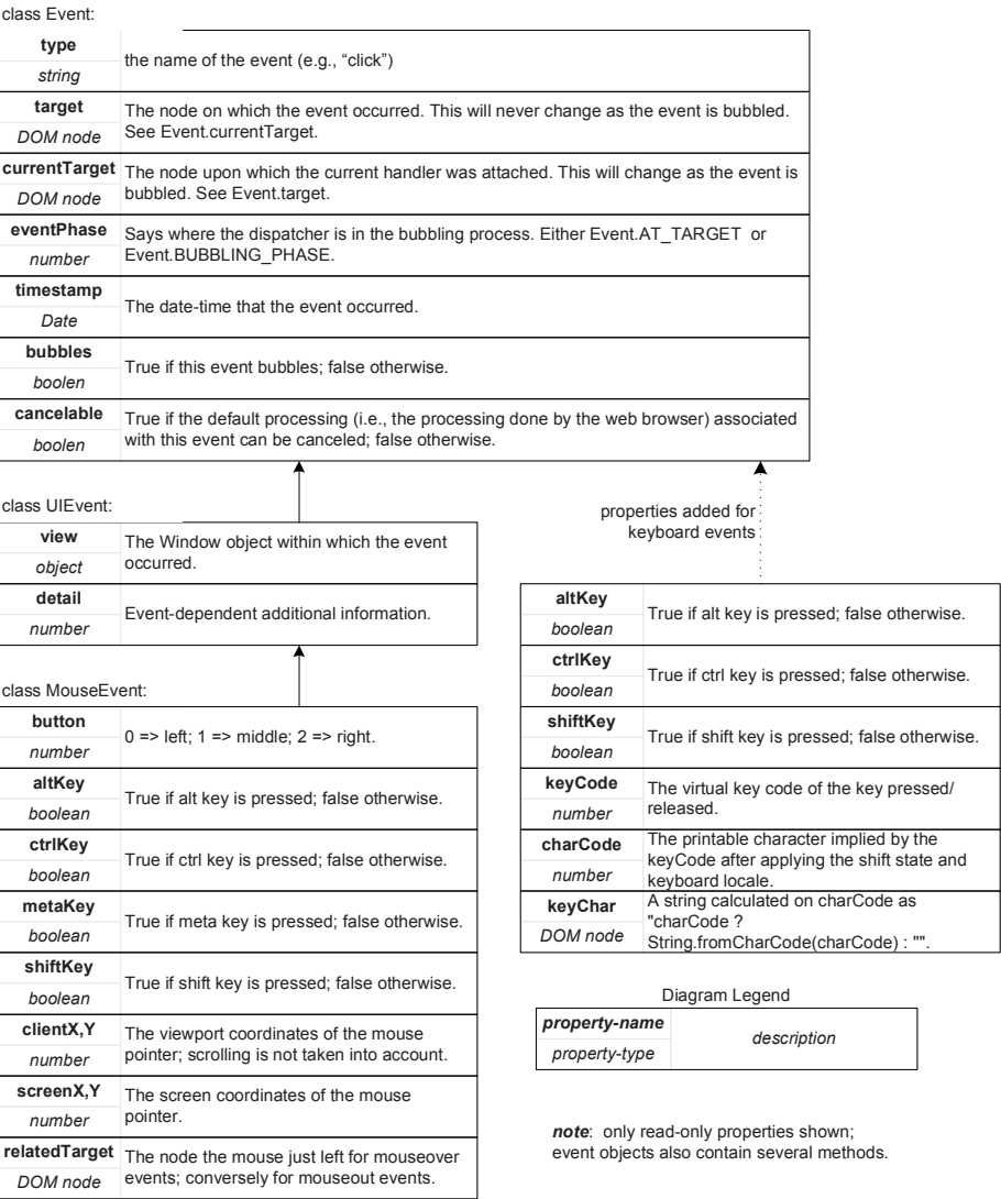
Figure 6.2: The event interfaces
