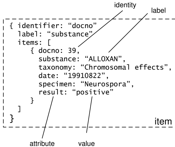
Figure 10.2: A dojo.data.ItemFileReadStore data source
